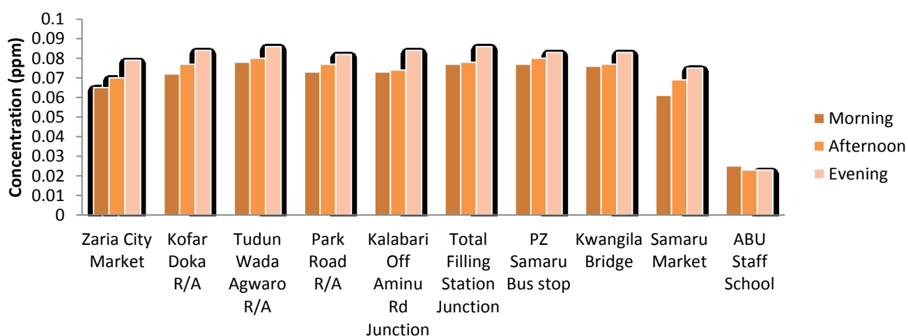
Figure 4. Mean Variation of Sulphur Dioxide ( \text{SO}_2 ) across periods at sampling points.
