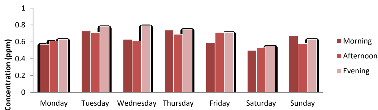
Fig. 7. Variation of Hydrogen Sulphide ( \text{H}_2\text{S} ) across periods at sampling days for Kwangila.
