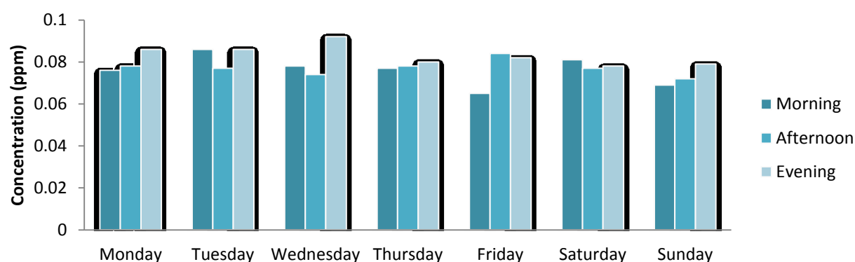
Fig. 6. Variation of Sulphur Dioxide ( \text{SO}_2 ) across periods at sampling days for Kwangila.
