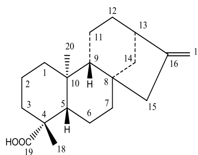
2. kaurenoic acid
