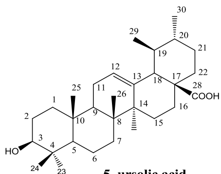
5. ursolic acid
