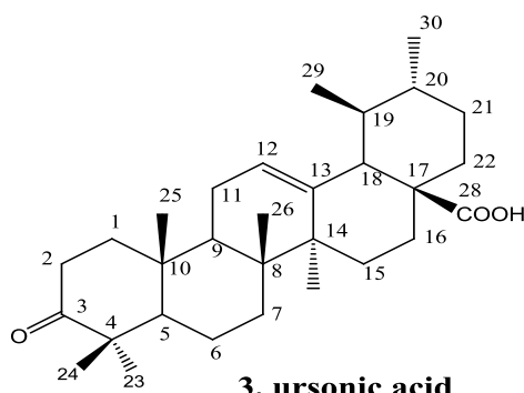
3. ursonic acid
