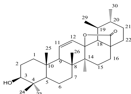
4. 3 \beta -hydroxy-11-ursen-28,13-olide
