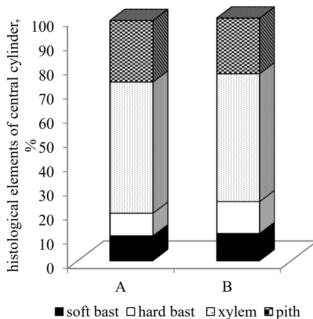
Fig. 2. The influence of \text{SO}_2 and \text{NO}_2 on the ratio of histological elements of the central cylinder of annual shoot stems of Salix alba L., %: A – reference area; B – test area
