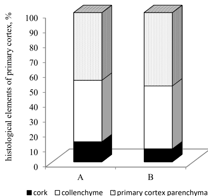
Fig. 1. The influence of \text{SO}_2 and \text{NO}_2 on the ratio of histological elements of primary cortex of annual shoot stems of Salix alba L., %: A – reference area; B – test area
