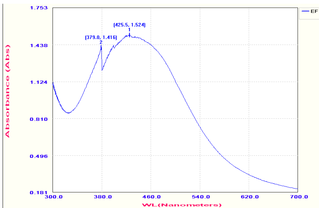
Fig.6: UV-Visible Spectra of AgNps of Endophytic fungus, Penicillium spinulosum
