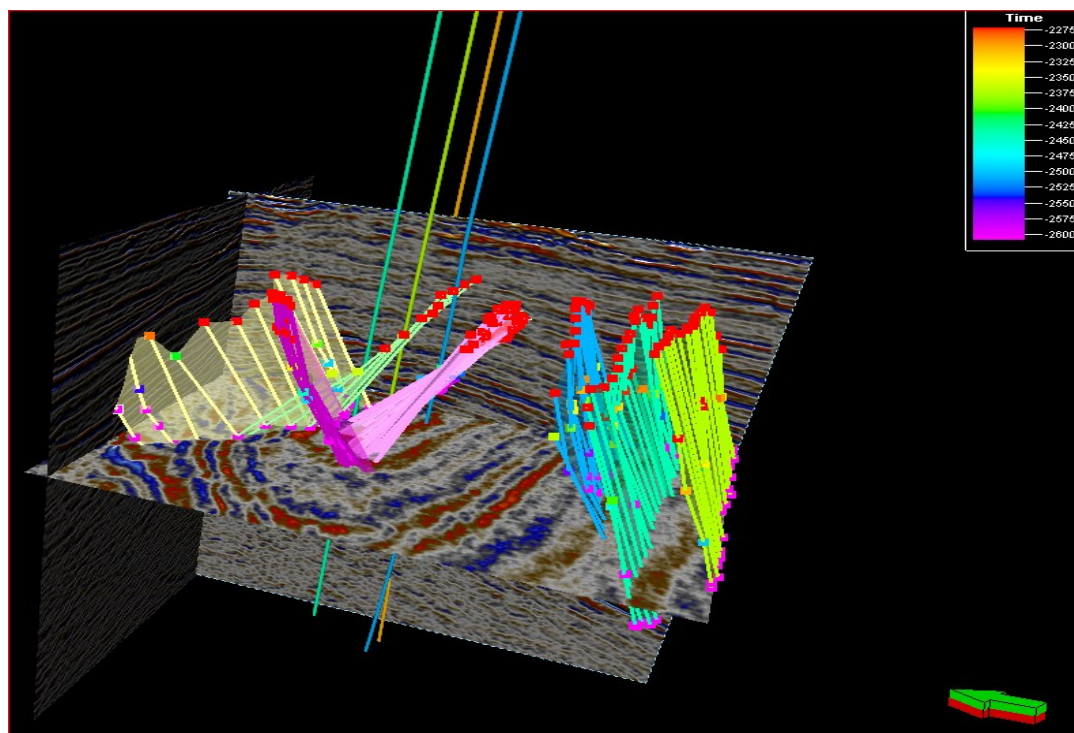
Fig.8. 3-D seismic section of inline 5713 with time slice showing the fault architecture of the field
