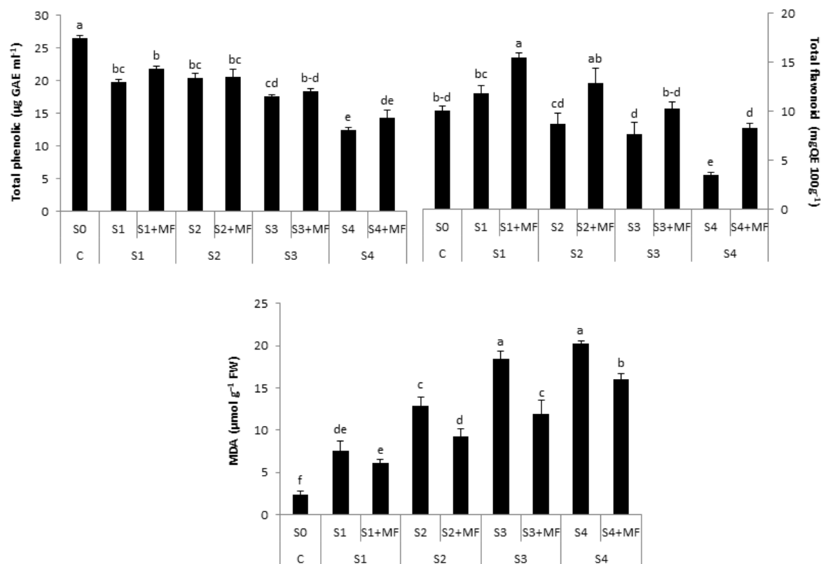
Figure 3. Effects of MF application on total phenolic, flavonoid, and MDA contents of guar under drought condition. Each value represents the mean of three replicates. For each parameter of each different letters are significantly different at p \leq 0.05 according to Student's t test
