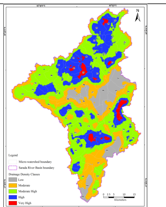
Figure 3: Drainage density map.
