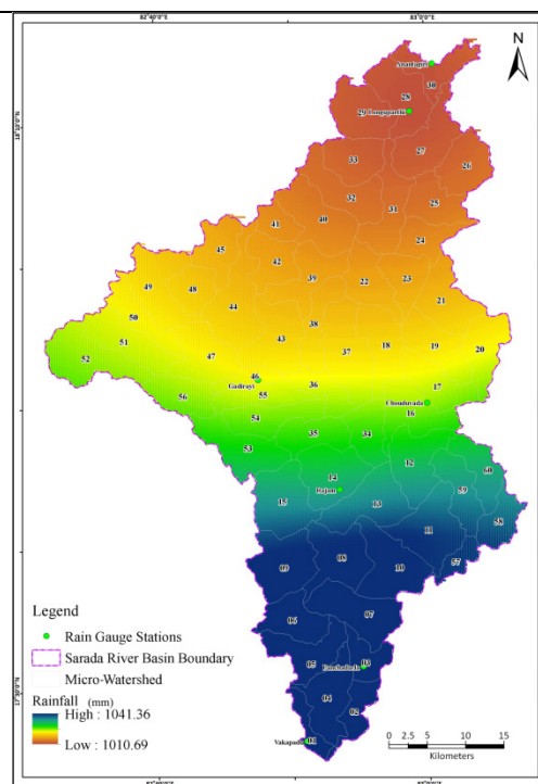
Figure 7: Distributin of avg. annual rainfall.
