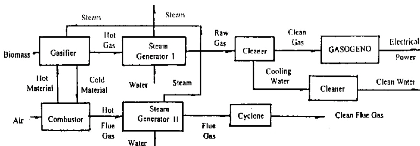
Figure 6. Application of biogas in internal combustion engine.
