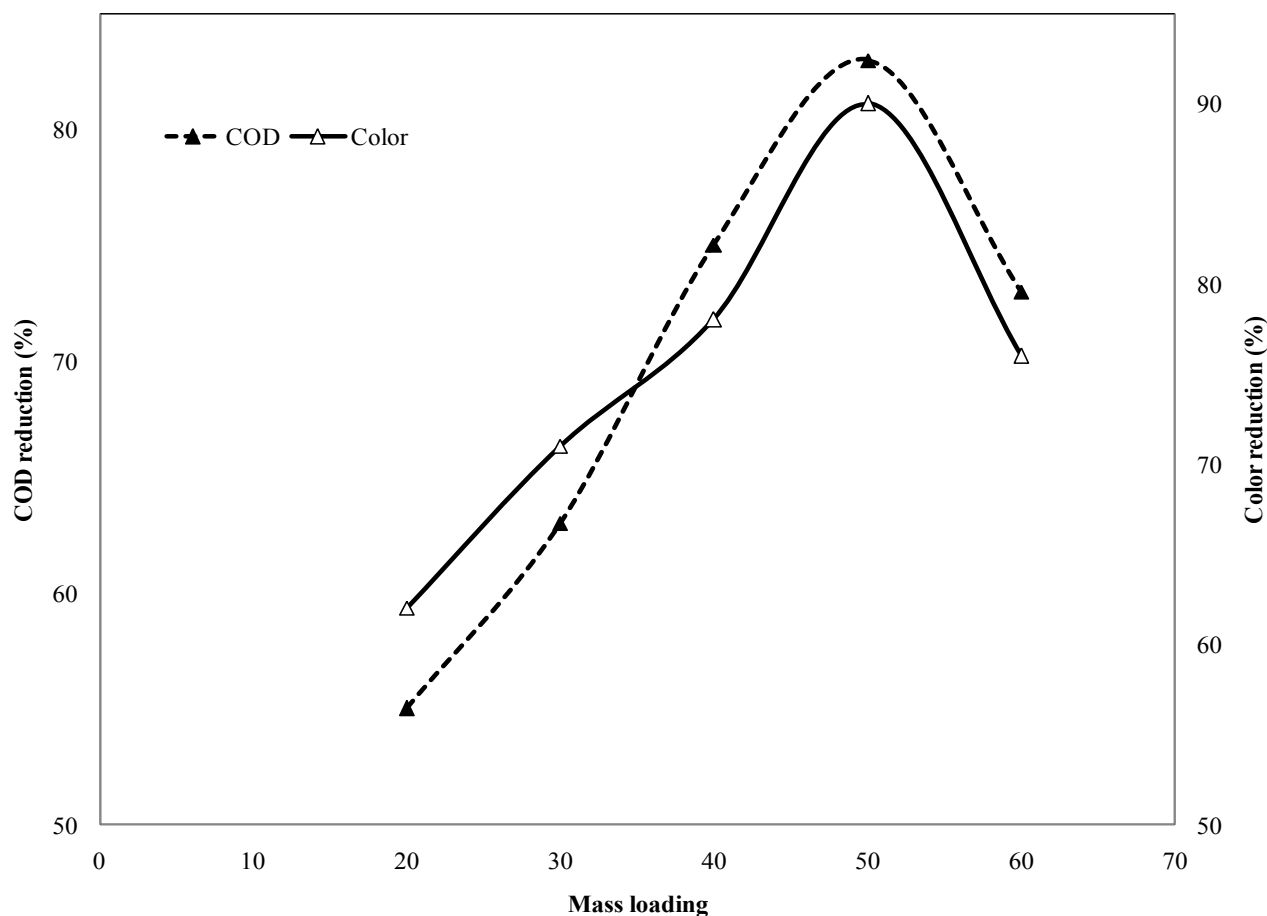
Fig. 4. Effect of mass loading on COD and color at optimum pH = 7.
