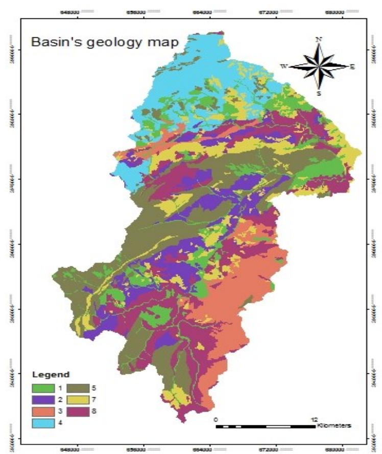
Figure 2. Basin's geology map.
